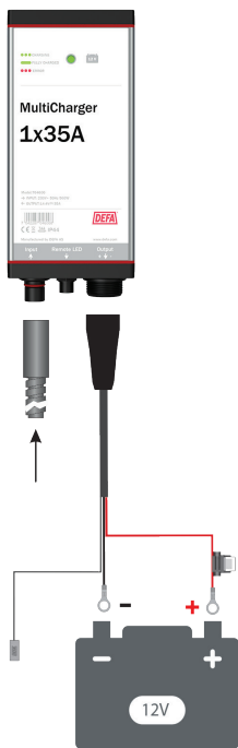
12V 1x35A
